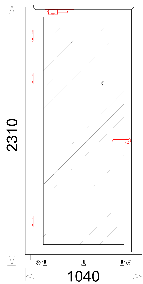
01 ELEVATION-Front wall
