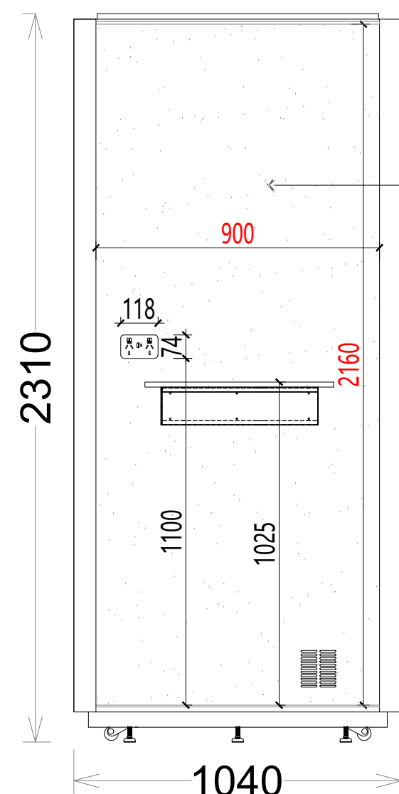
02 ELEVATION-Right wall
