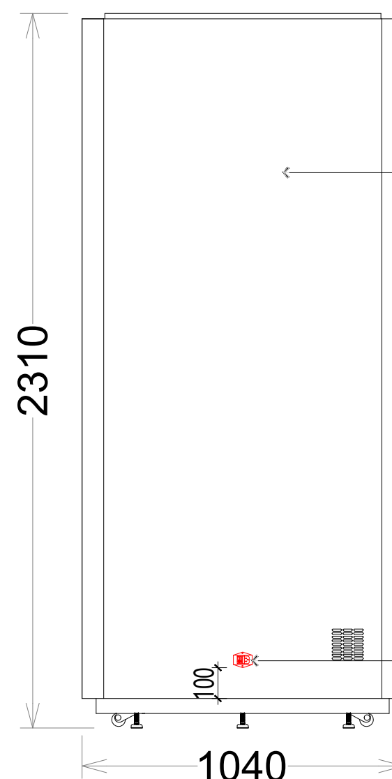
02 ELEVATION-Right wall
